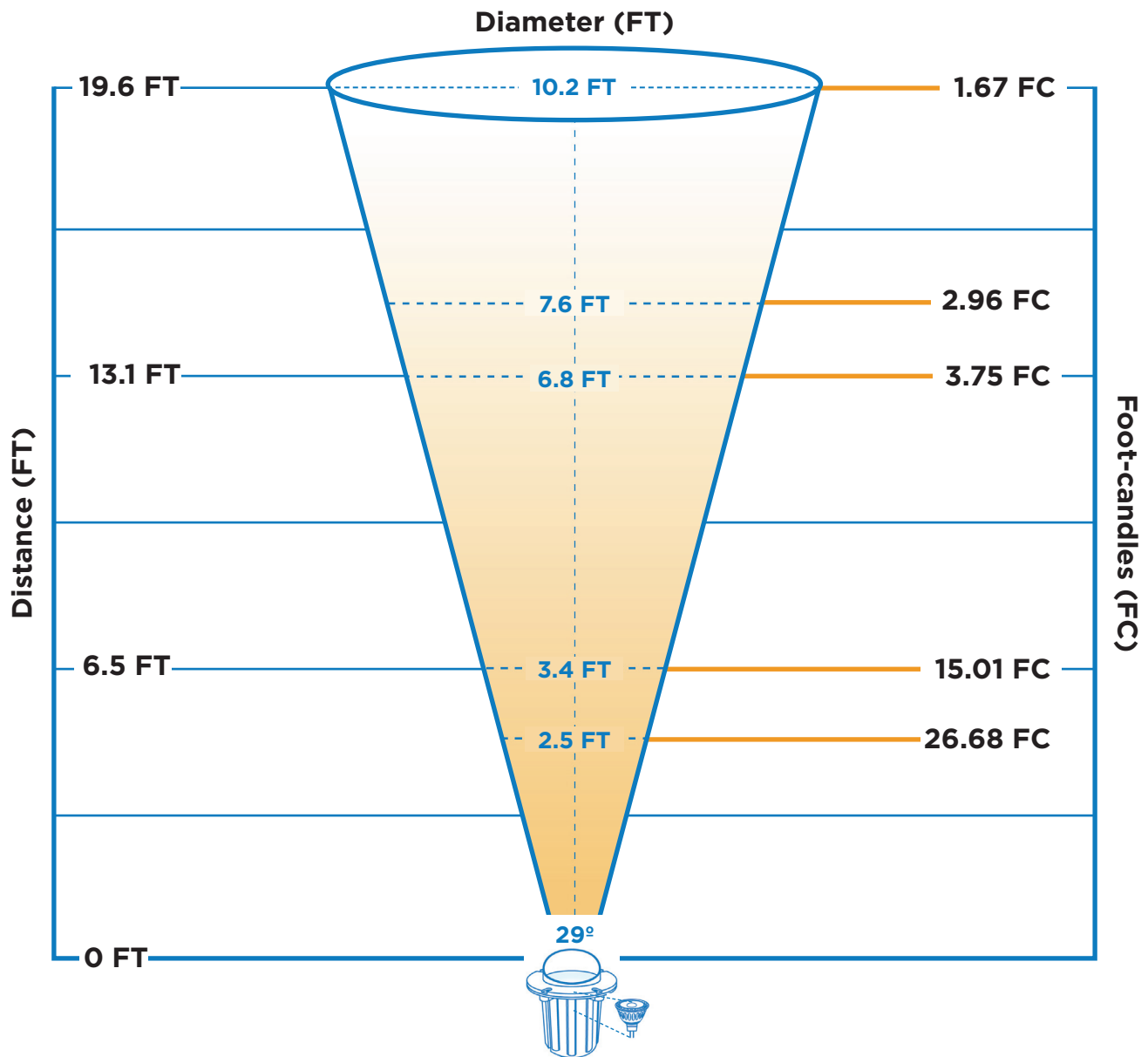
Lamp: LMR16-LED6W-F
