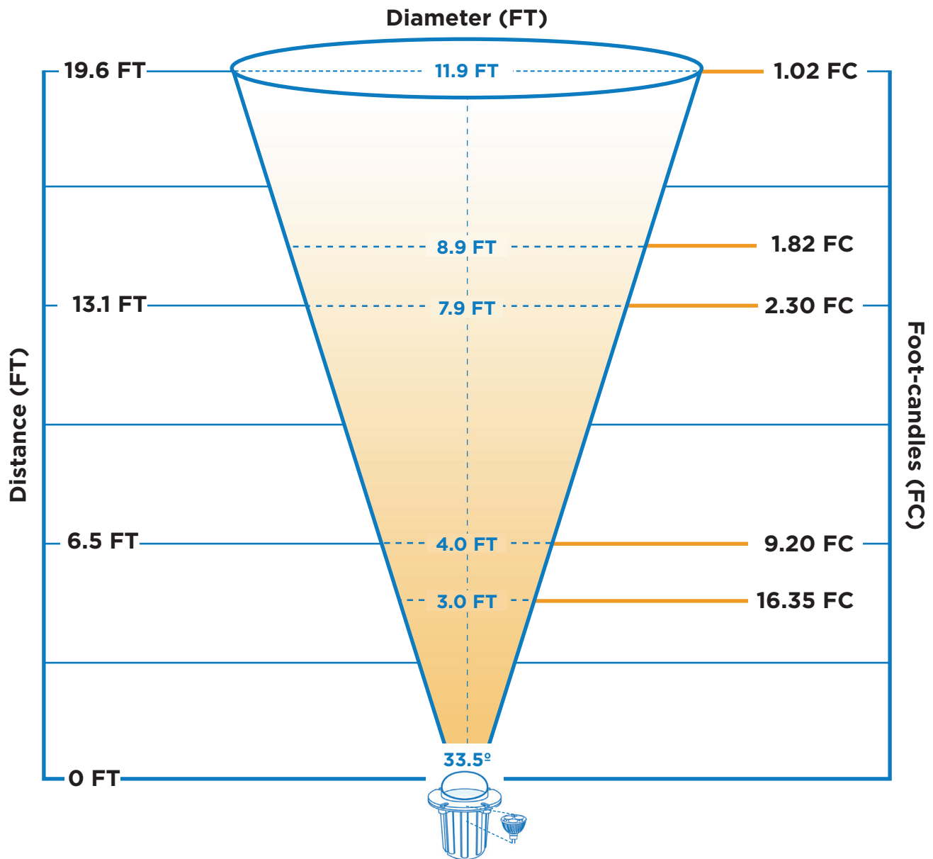
Lamp: LMR16-LED5W-F
