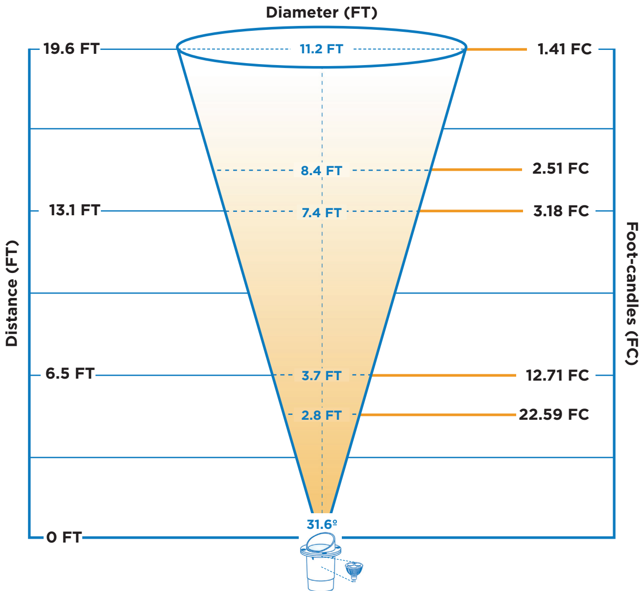
Lamp: LMR16-LED5W-F
