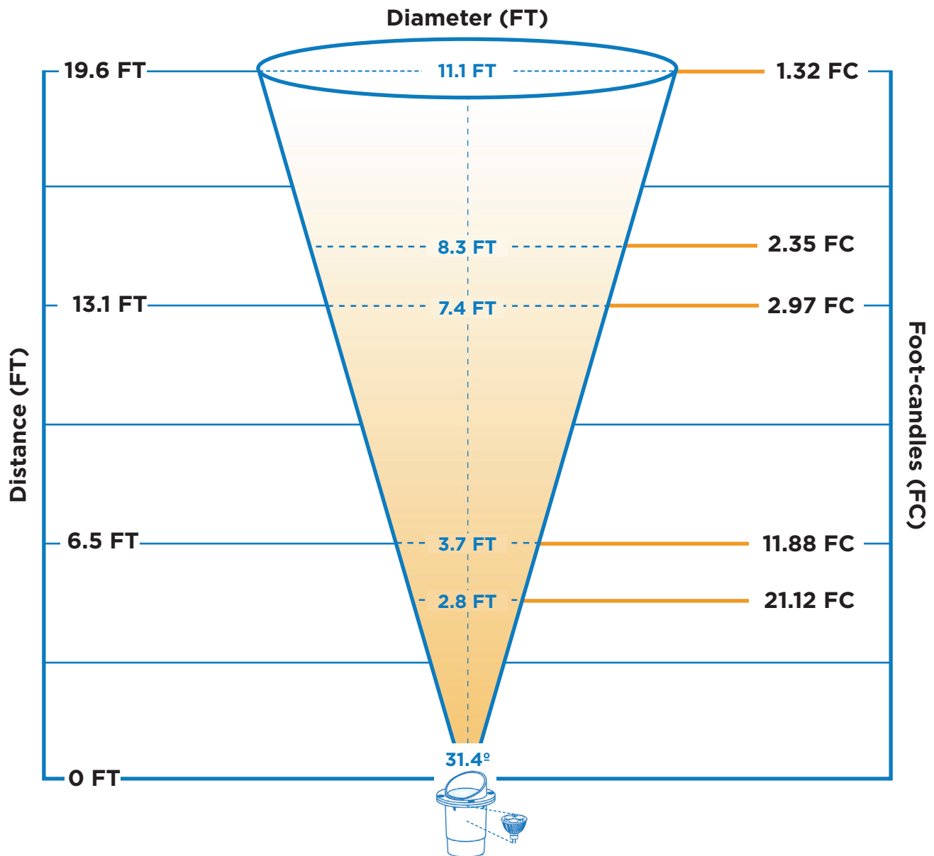
Lamp: LMR16-LED4W-F
