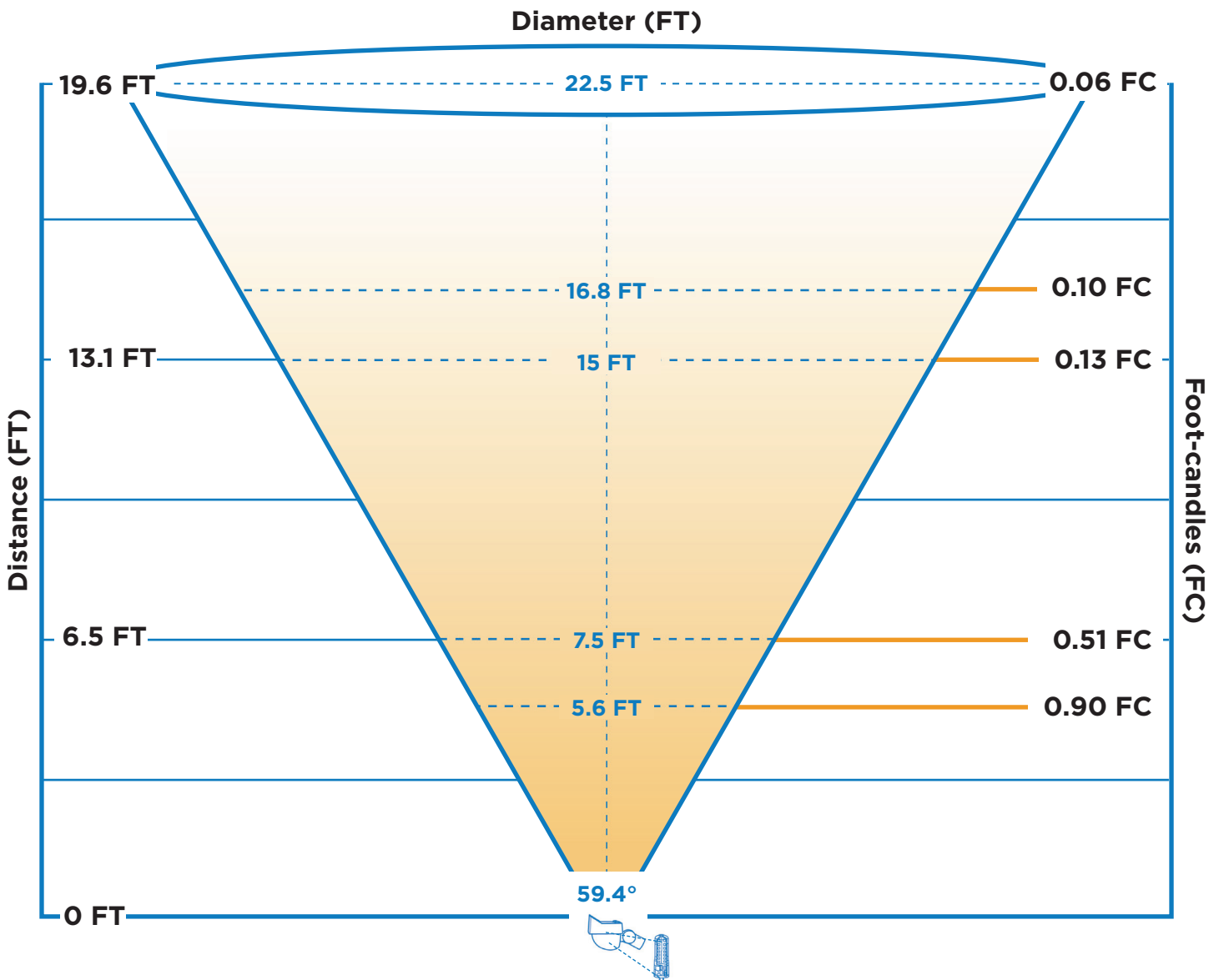
Lamp: LBIPIN-LED350lm
