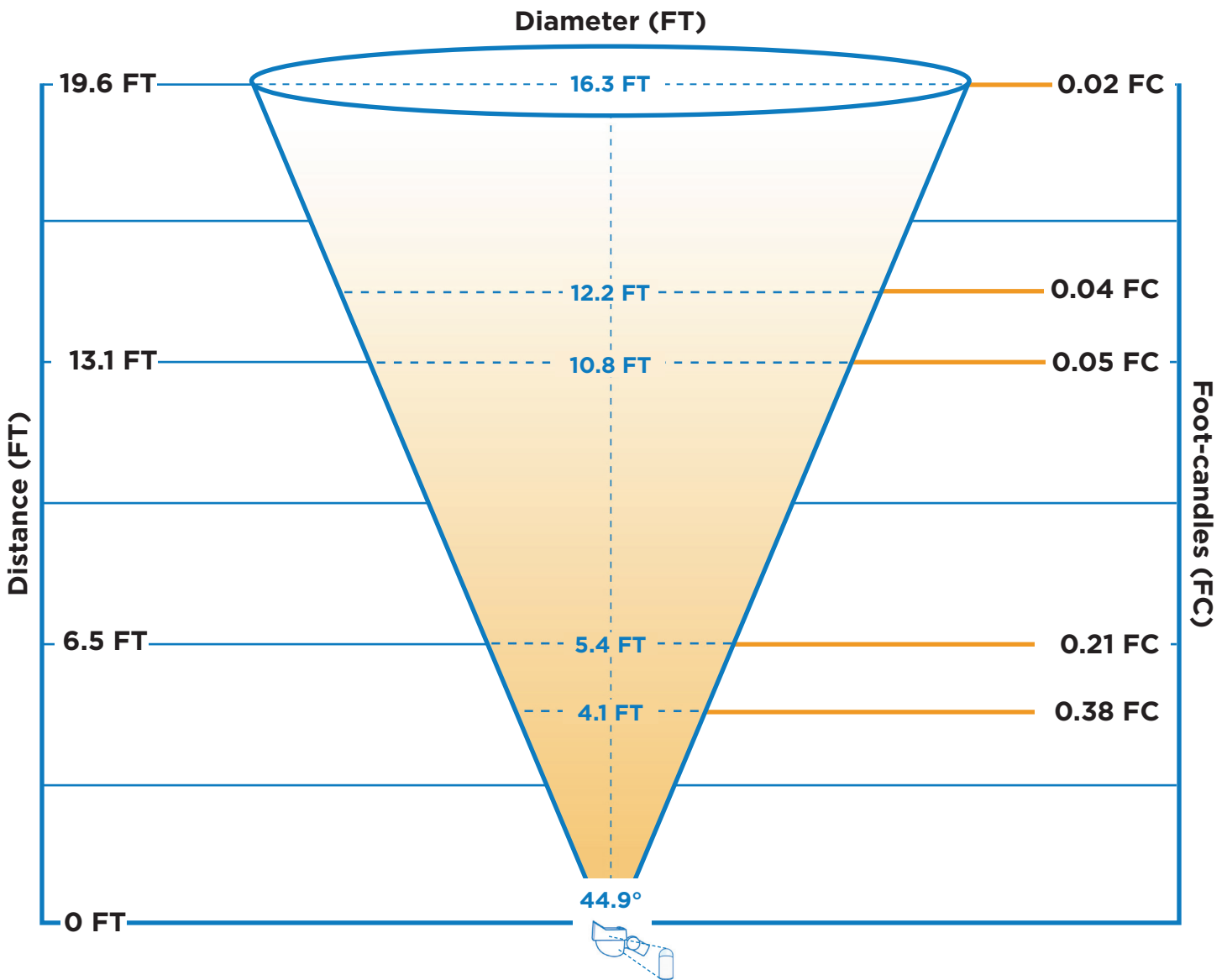
Lamp: BT-ALLY-G4
