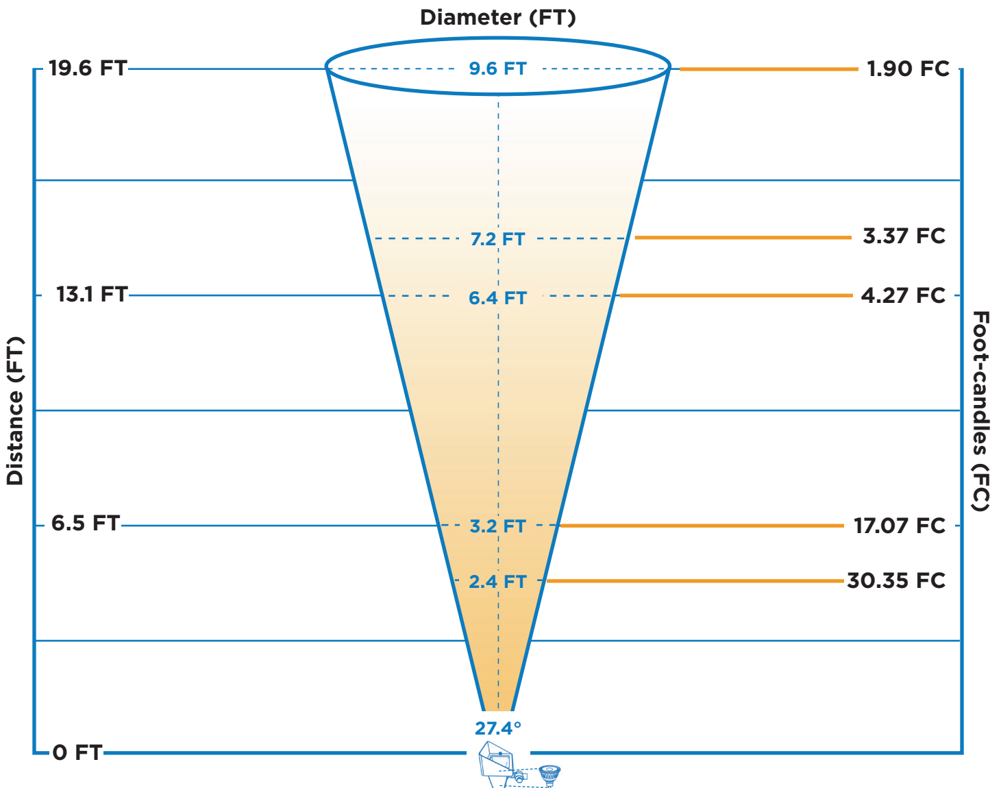
Lamp: LMR16-LED6W-F
