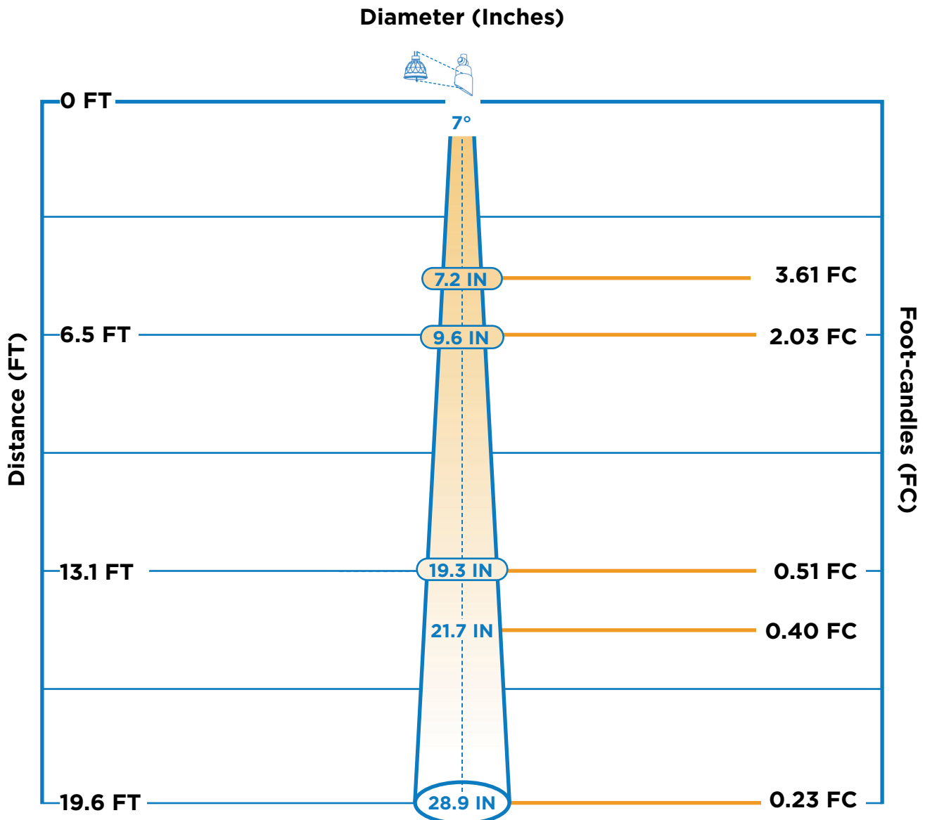
Lamp: BT-ALLY-MR16
