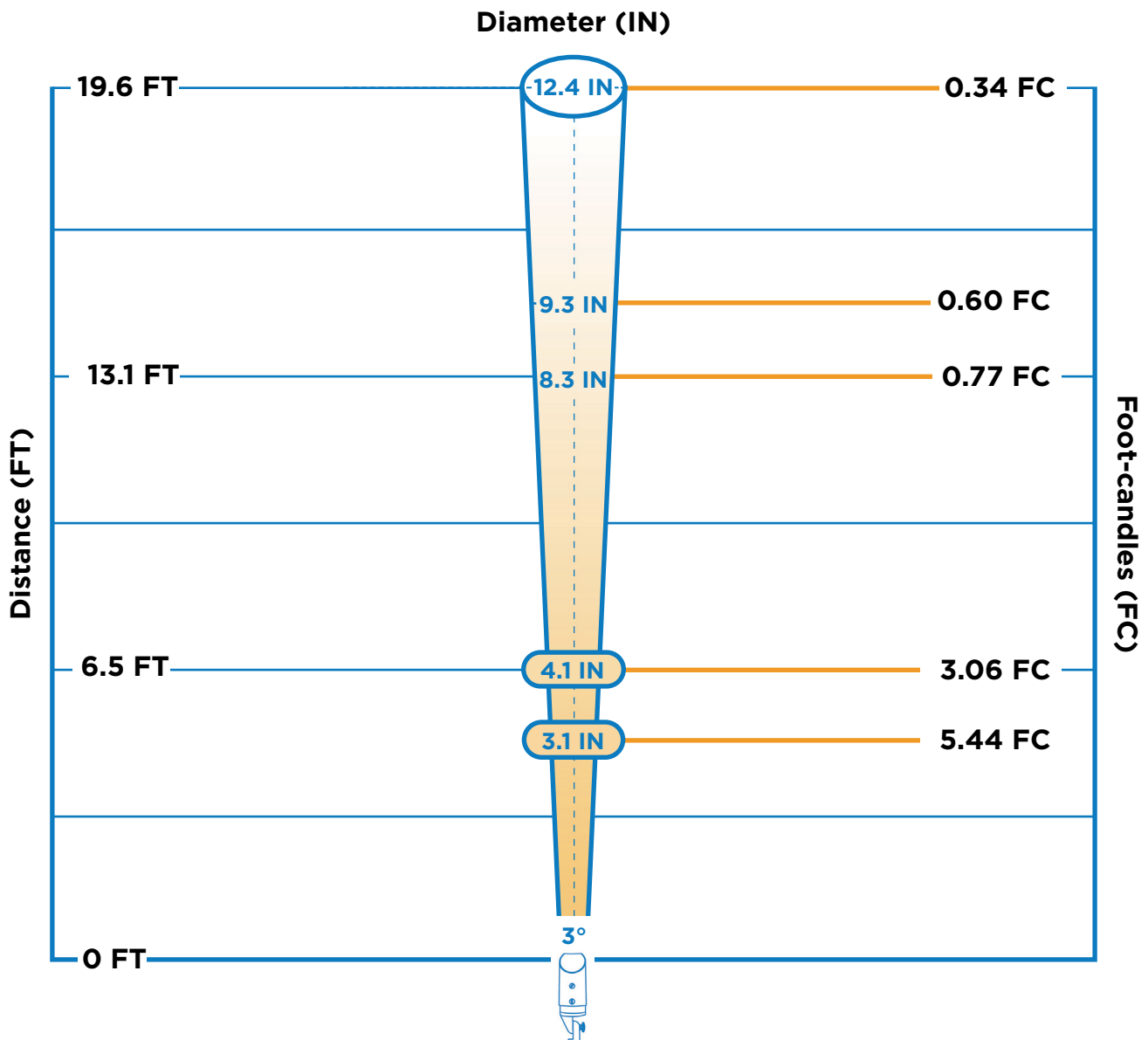
Lamp: INTEGRATED BT MODULE
