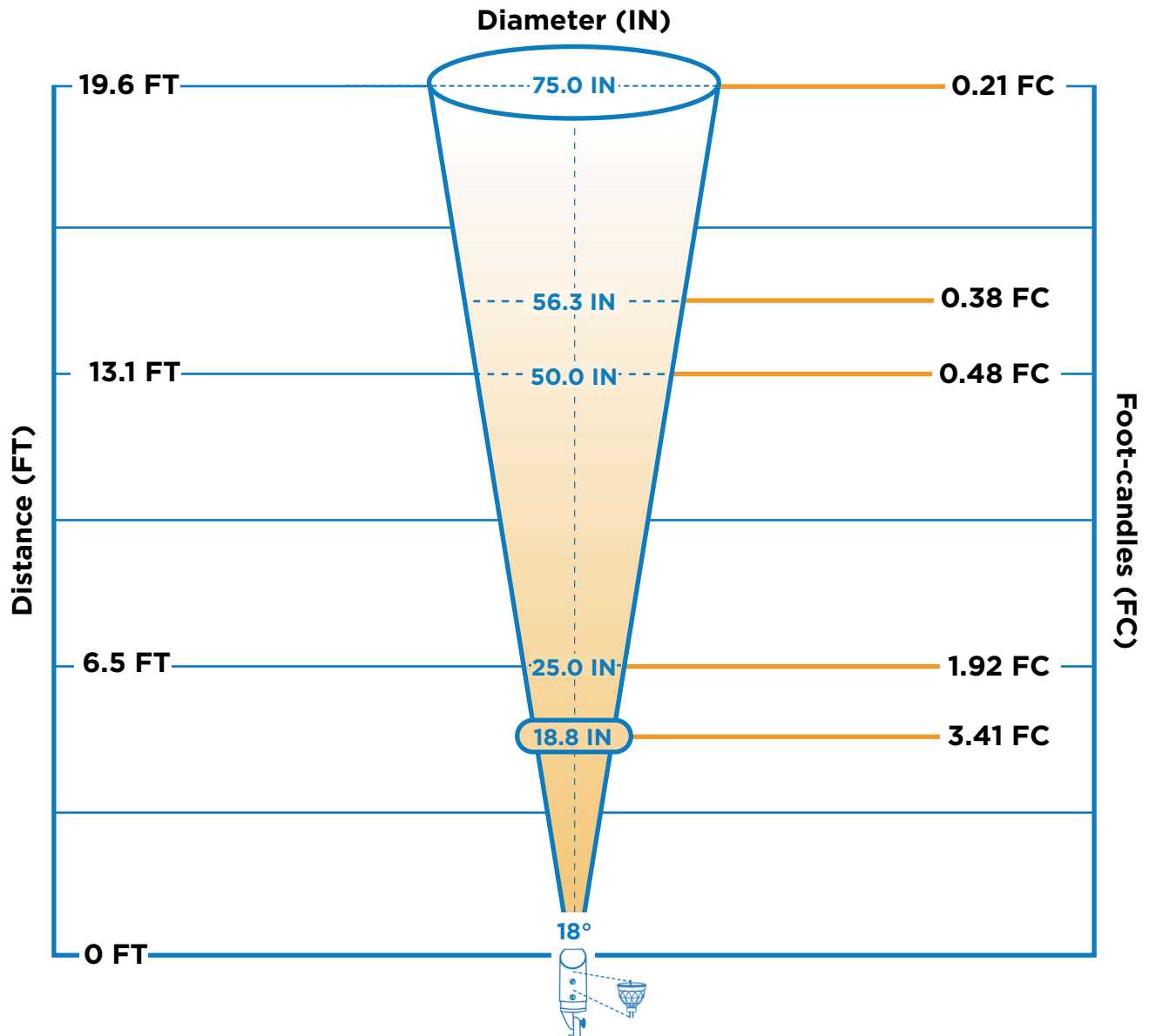
Lamp: BT-ALLY-MR16
