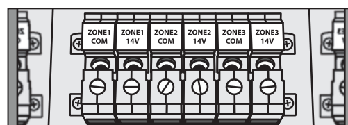
Zone labeled it2 terminal lugs
